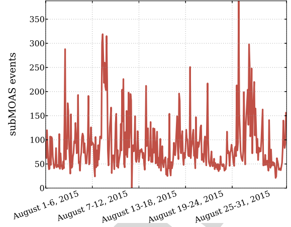
Fig. 4. subMOAS events observed with our experiment.
